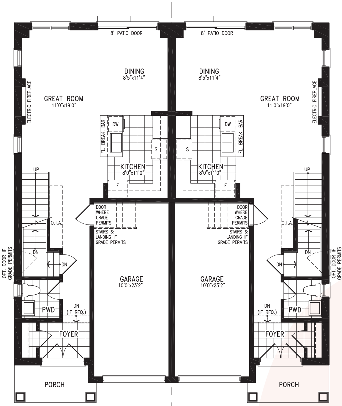
Elevation A1 GROUND FLOOR
