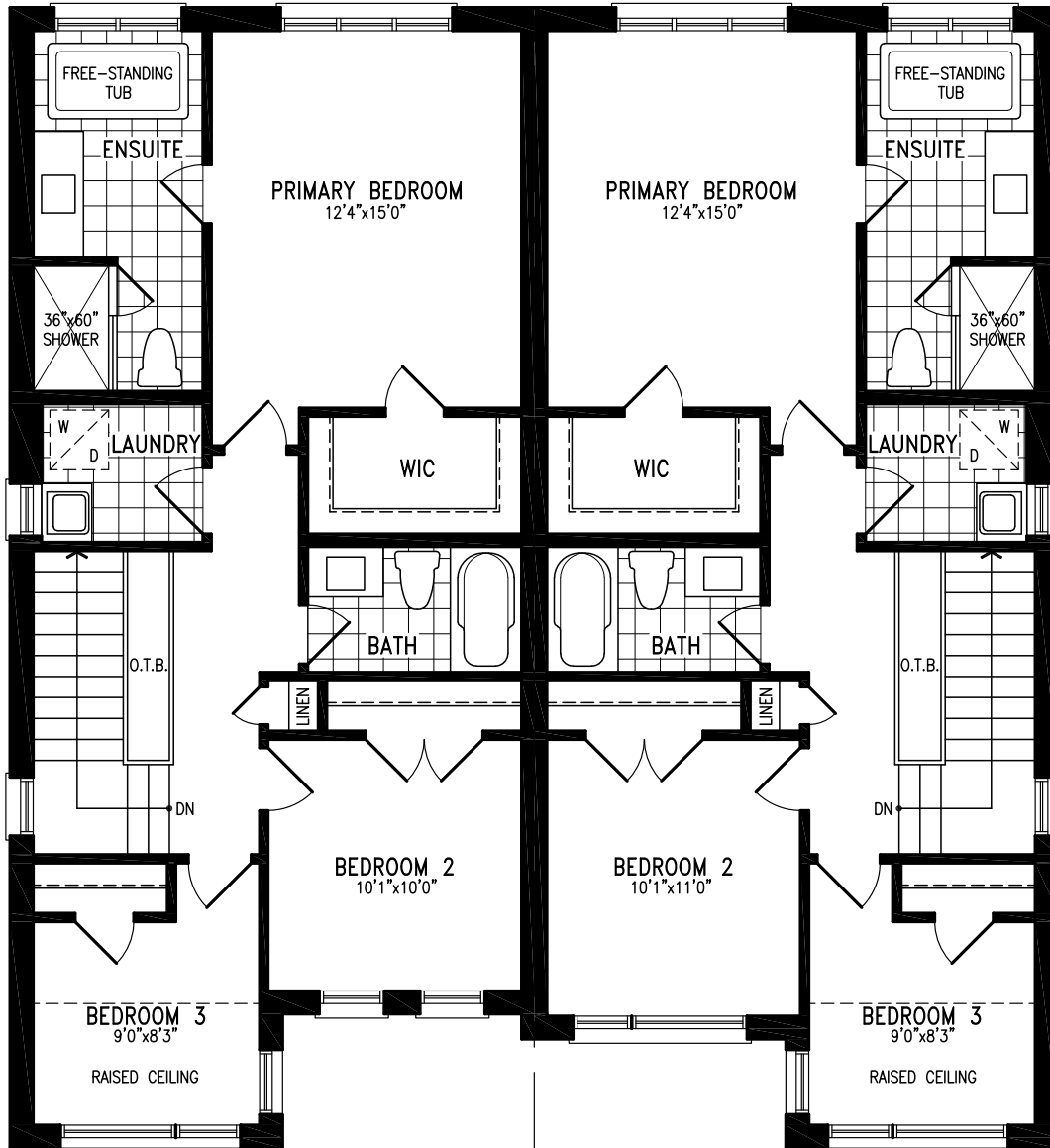
Elevation C1 SECOND FLOOR
