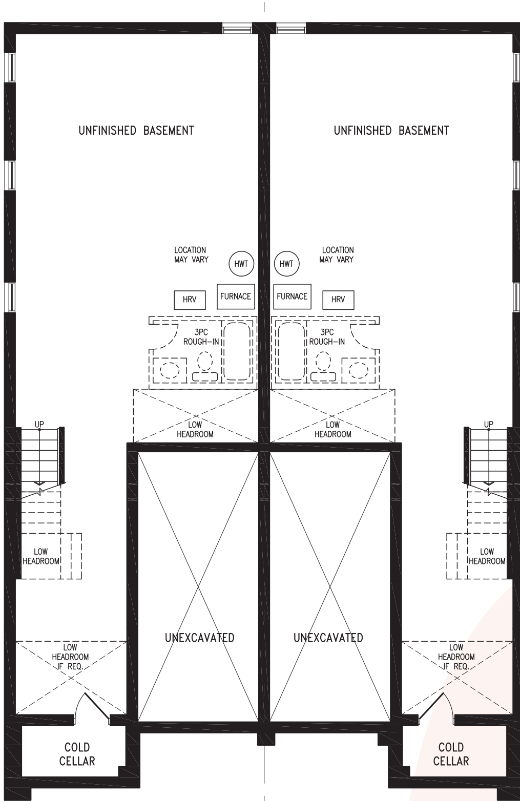
Elevation C1 BASEMENT
