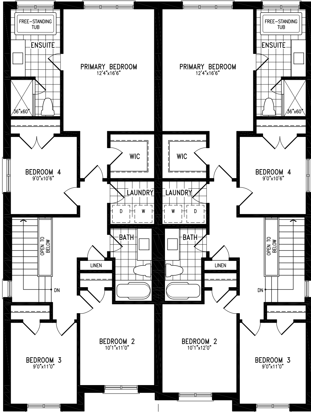
Elevation A1 SECOND FLOOR
