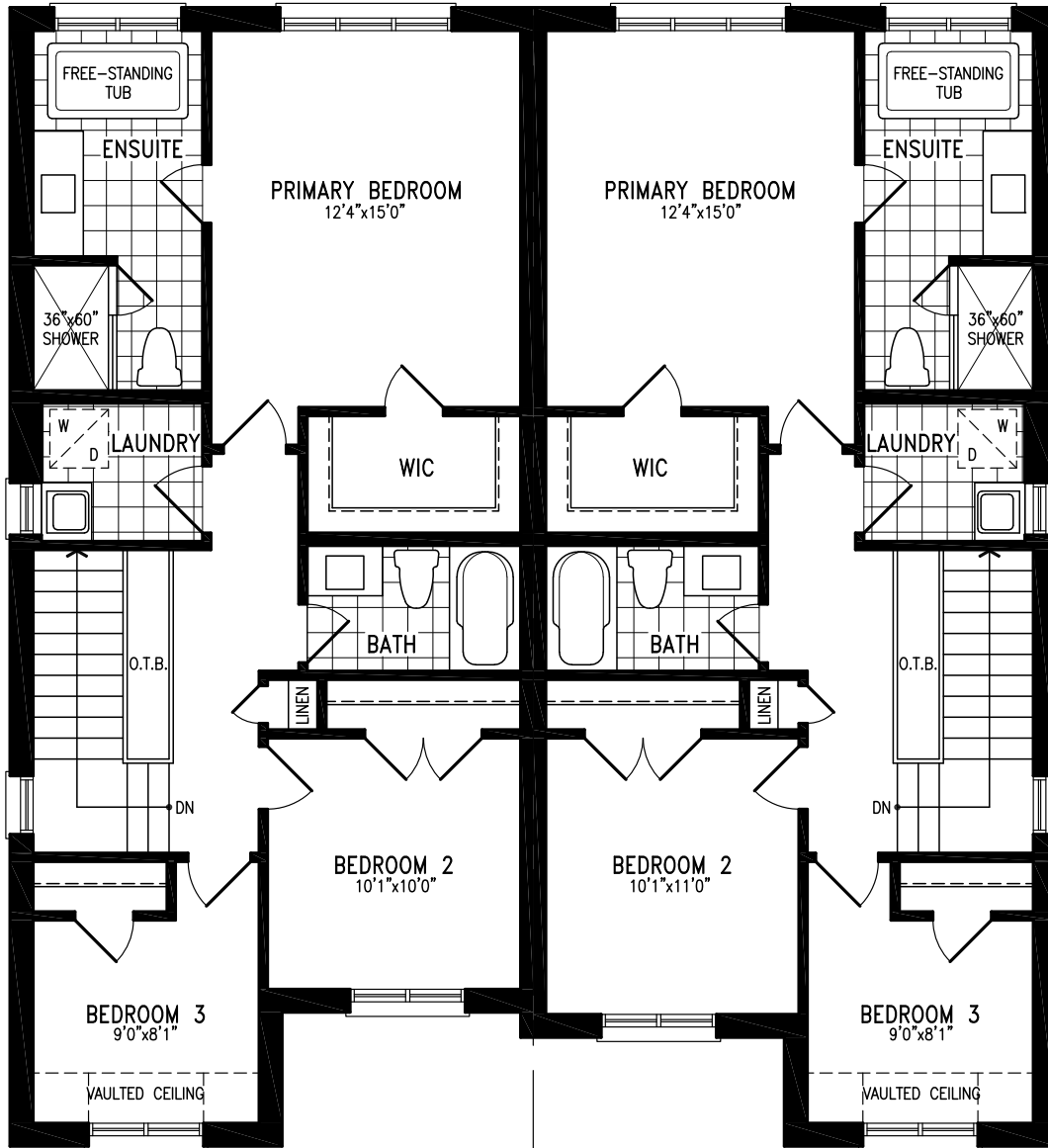
Elevation B1 SECOND FLOOR
