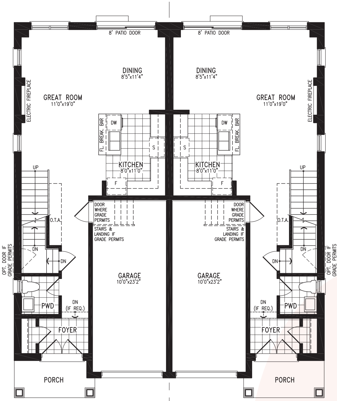
Elevation B1 GROUND FLOOR
