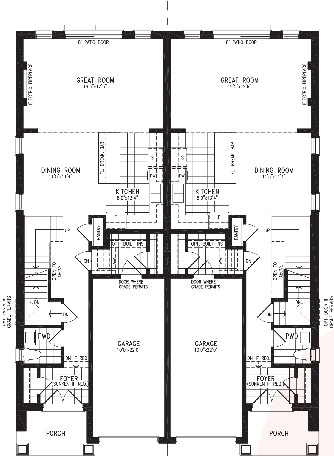
Elevation A1 GROUND FLOOR
