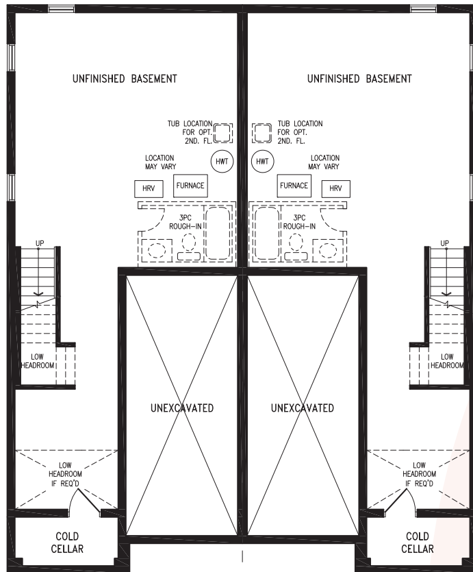
Elevation B1 BASEMENT
