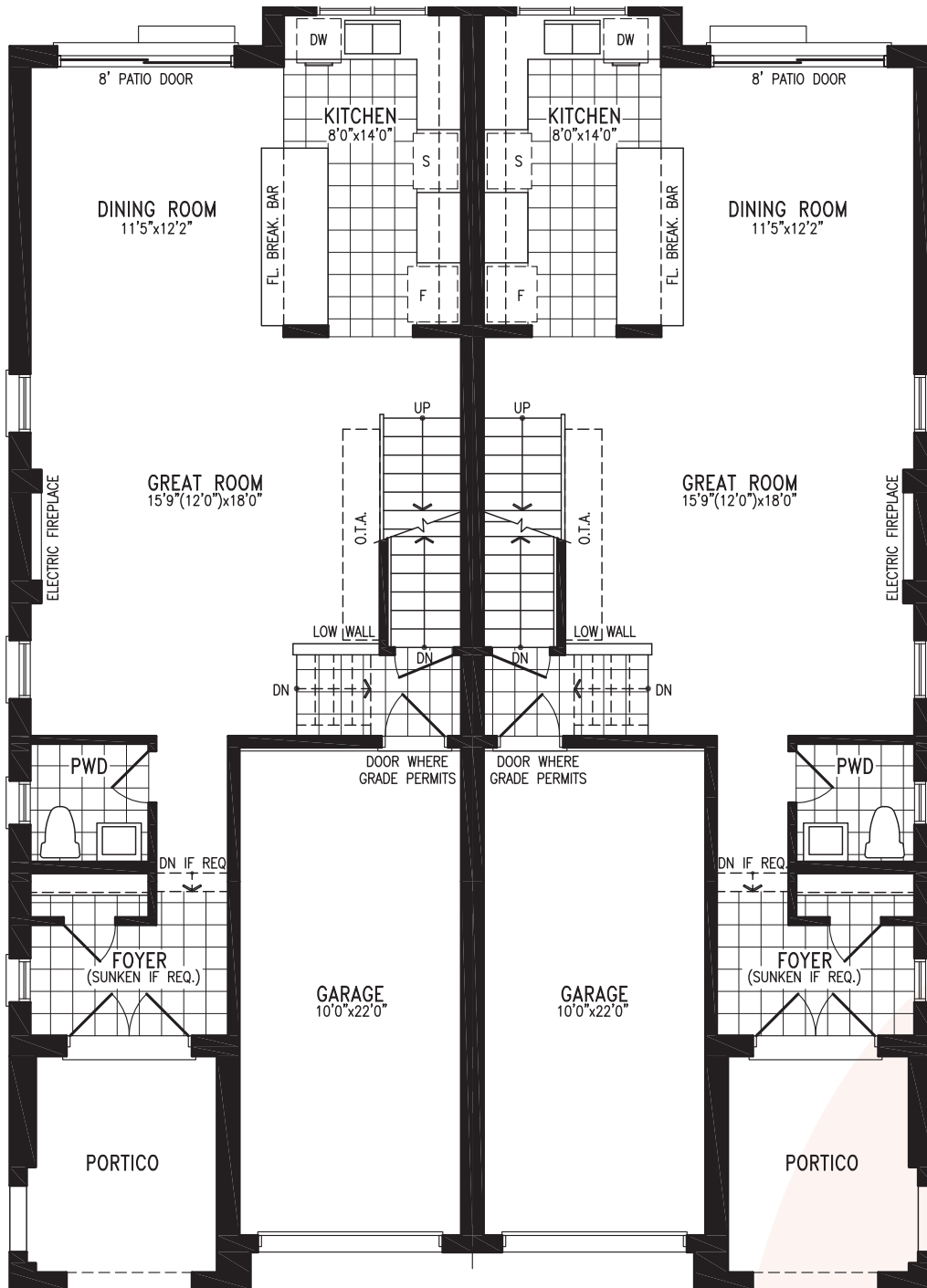
Elevation B1 GROUND FLOOR
