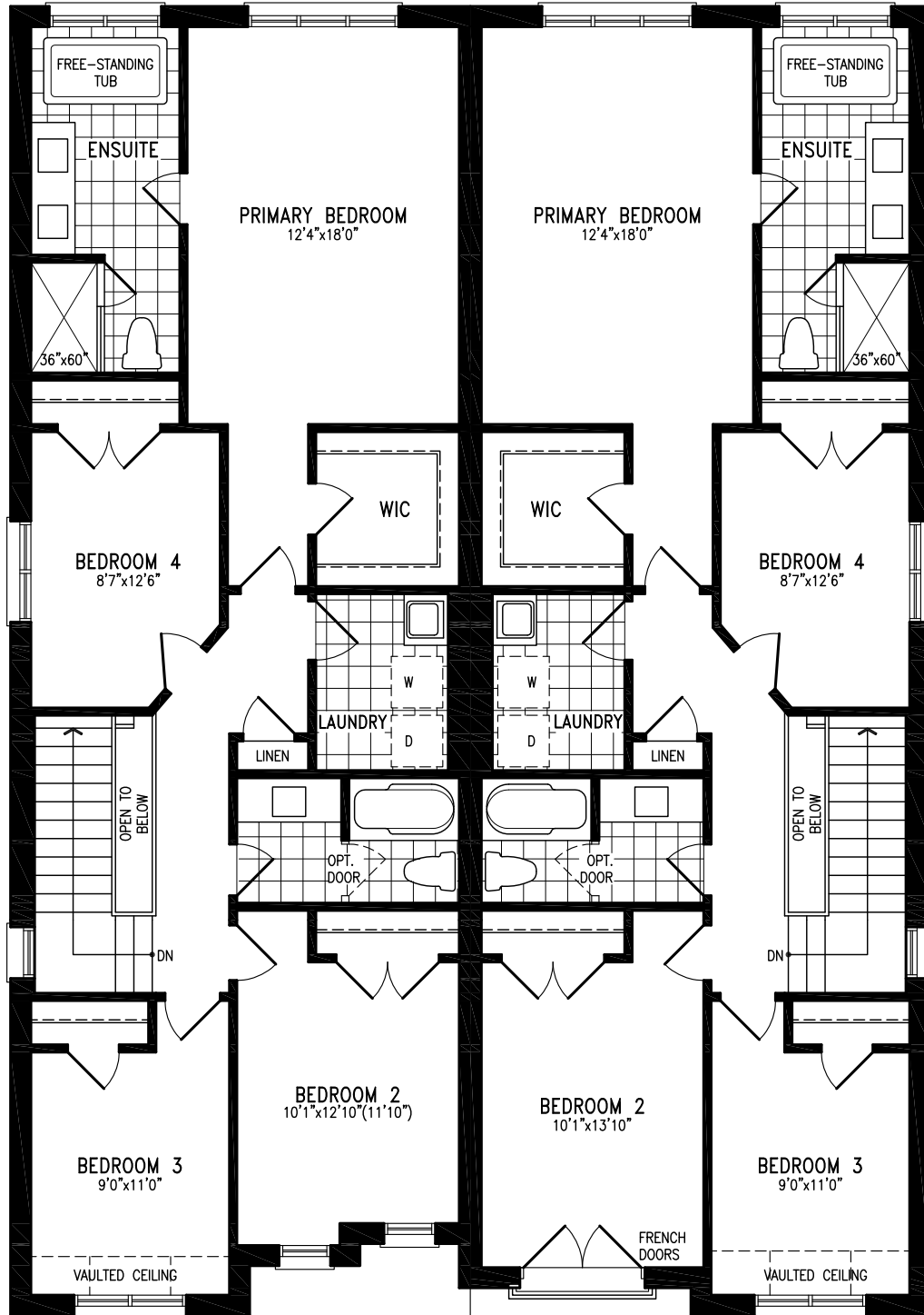
Elevation B1 SECOND FLOOR
