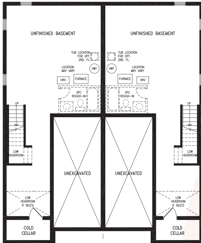
Elevation A1 BASEMENT
