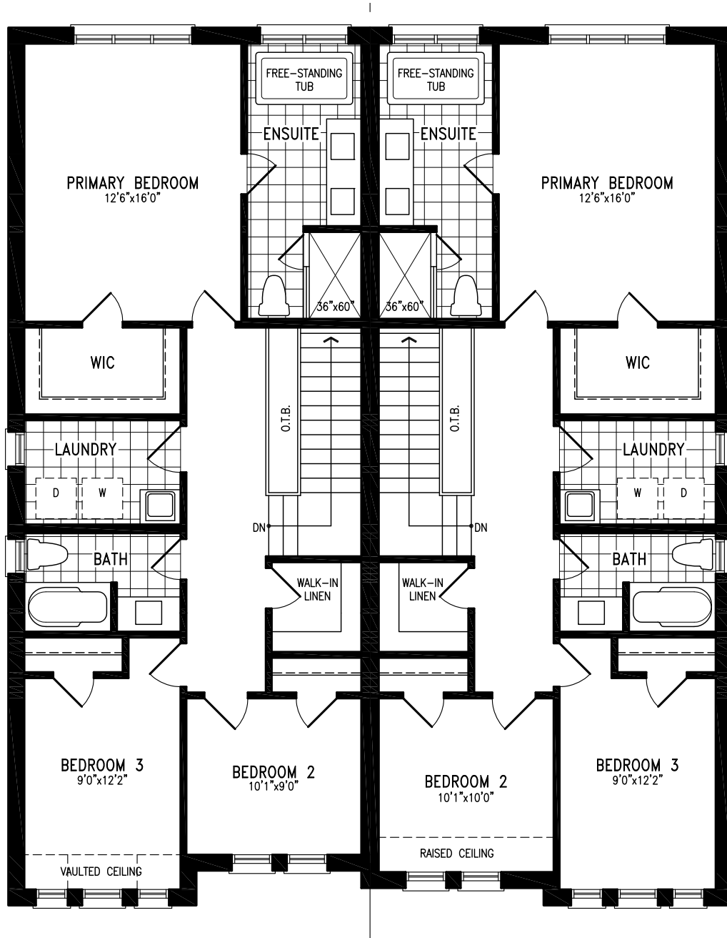
Elevation B1 SECOND FLOOR
