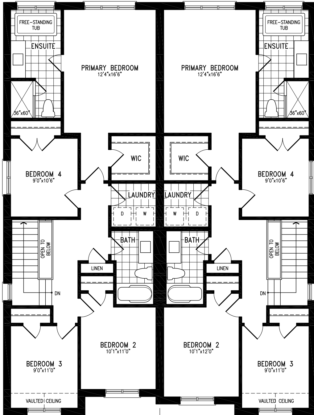
Elevation B1 SECOND FLOOR
