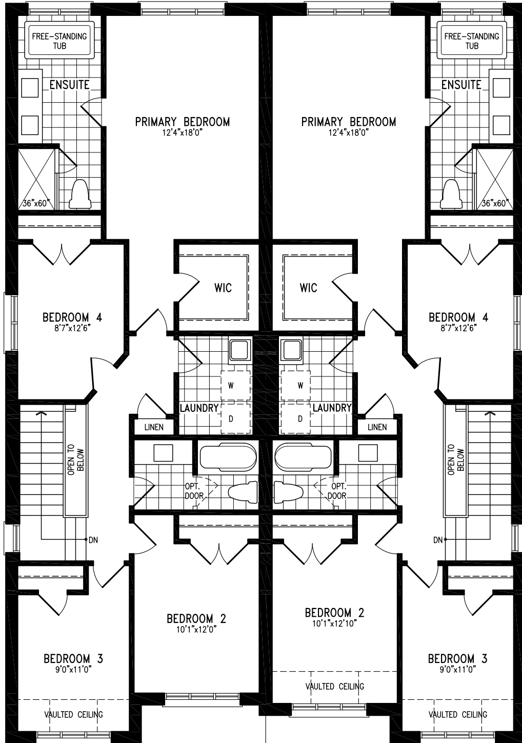
Elevation A1 SECOND FLOOR
