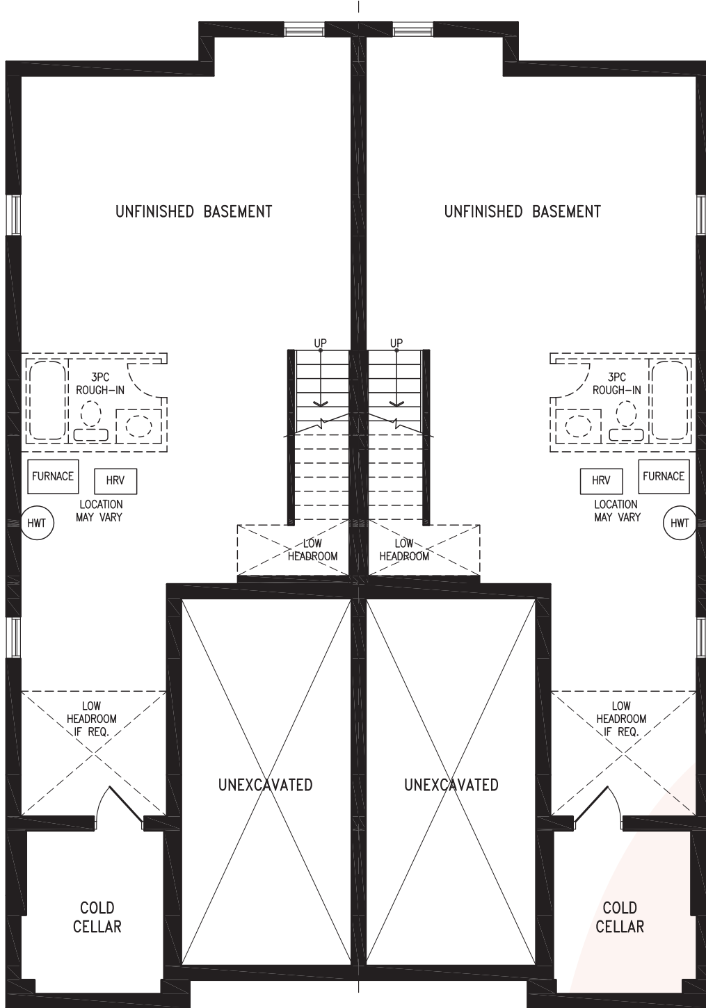
Elevation C1 BASEMENT
