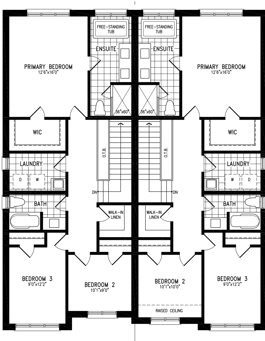
Elevation A1 SECOND FLOOR
