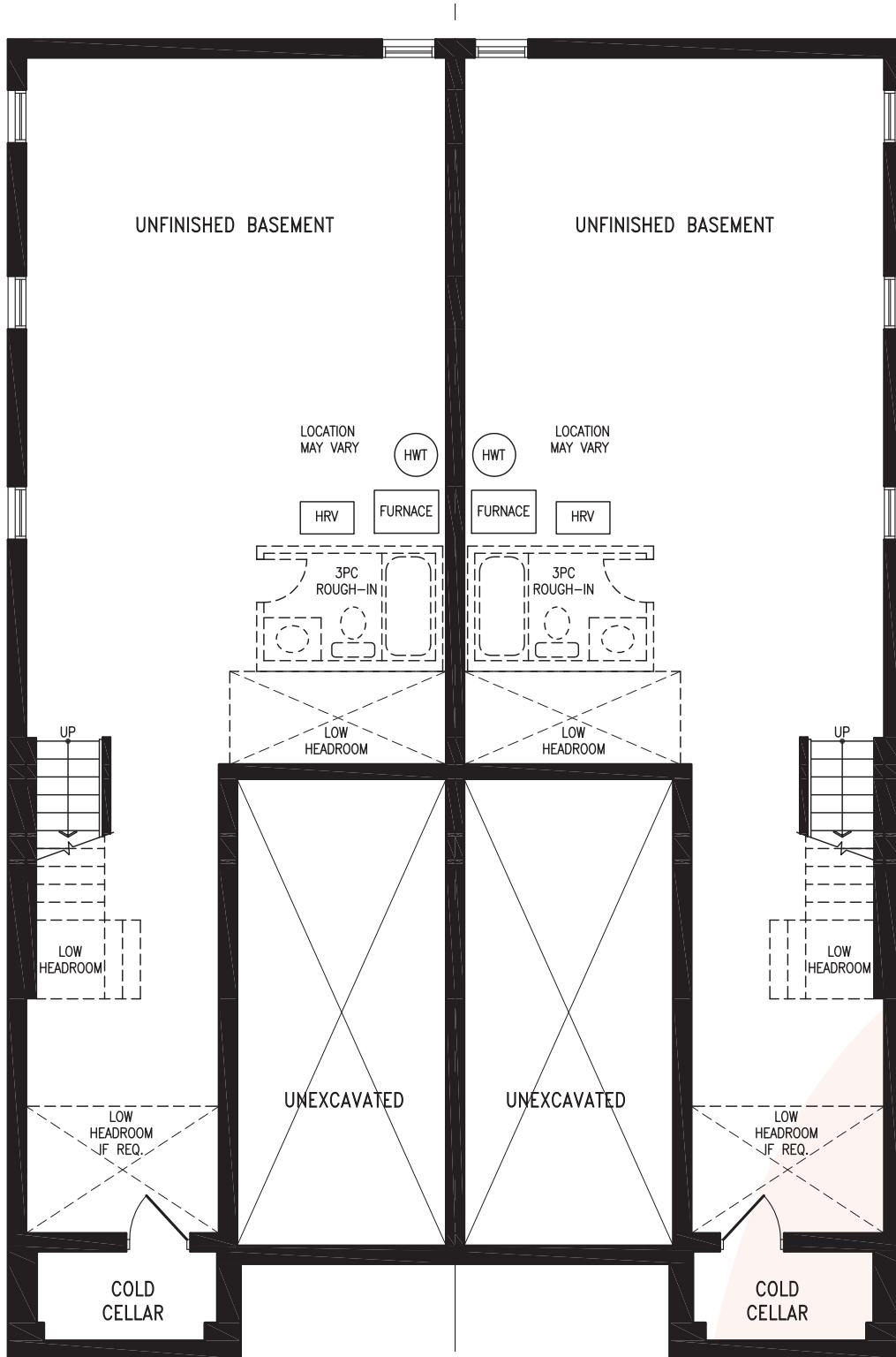
Elevation A1 BASEMENT
