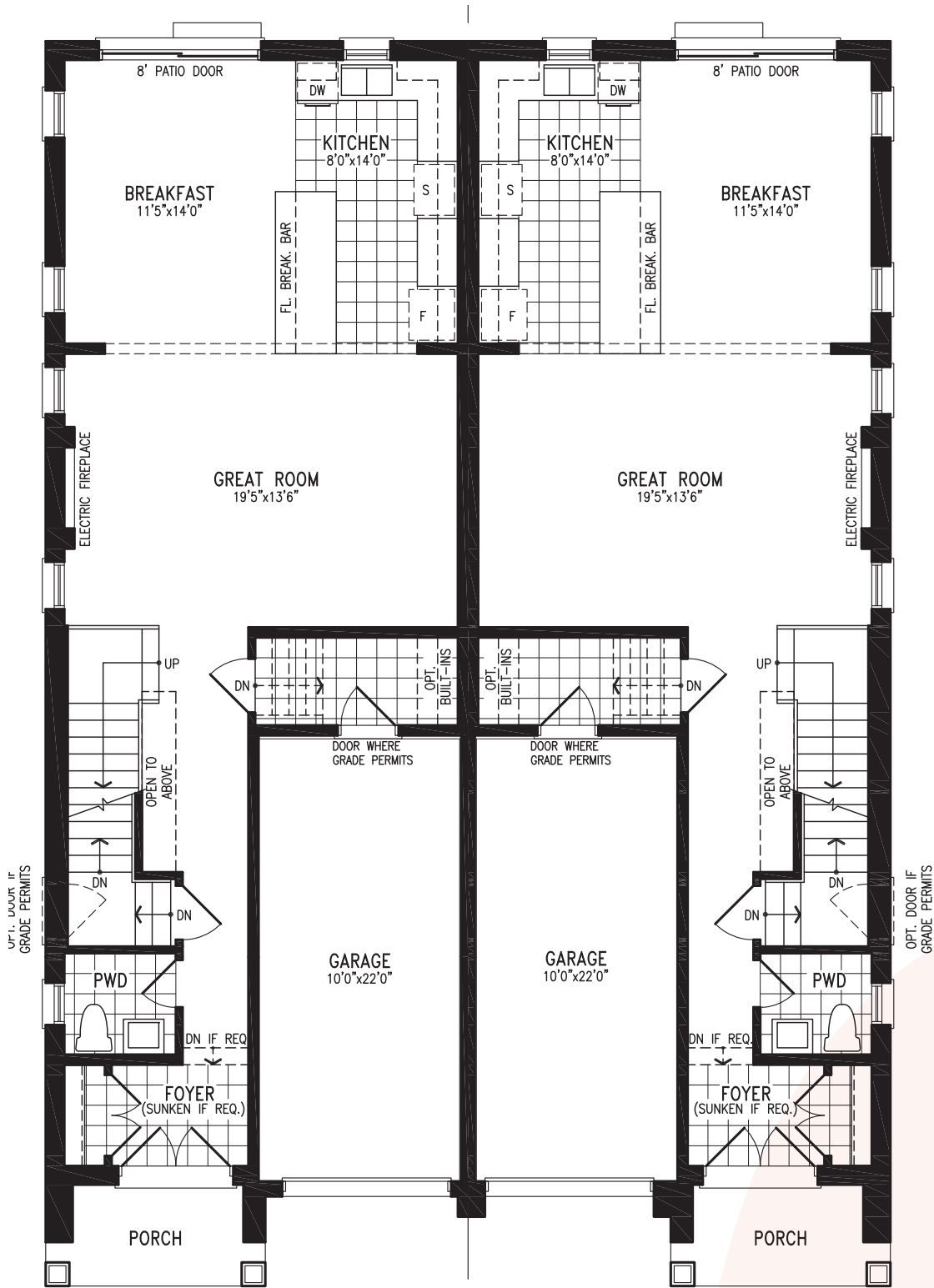
Elevation B1 GROUND FLOOR
