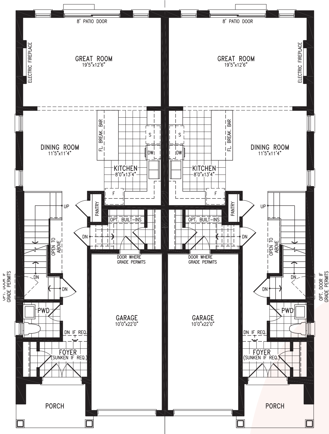
Elevation B1 GROUND FLOOR
