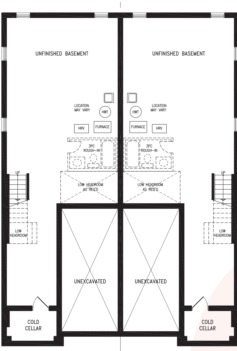
Elevation B1 BASEMENT
