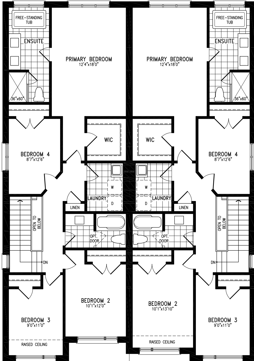
Elevation C1 SECOND FLOOR
